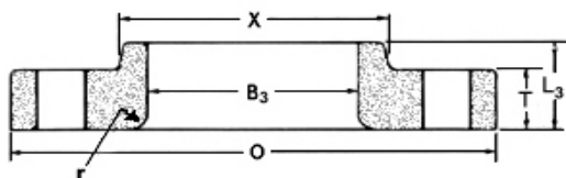
Lap Joint
