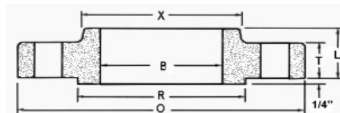
Slip-On
